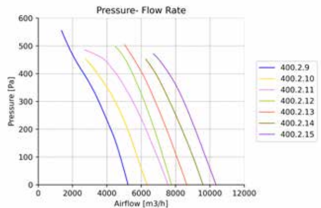
Ø400 / 6-8-10 Blade
